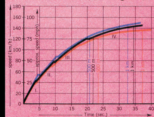
Acceleration and average speed for 1 km (.621 mile) (standing start)
